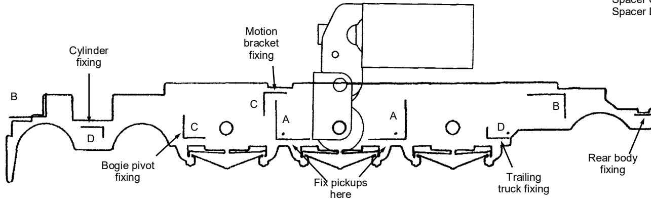
Sketch 5 Suggested pick up arrangement
