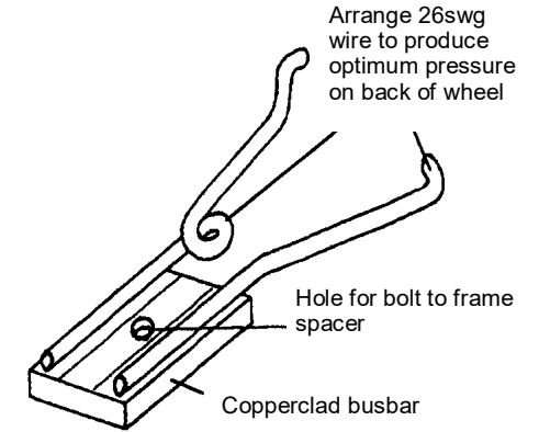
Sketch 5 Suggested pick up arrangement
