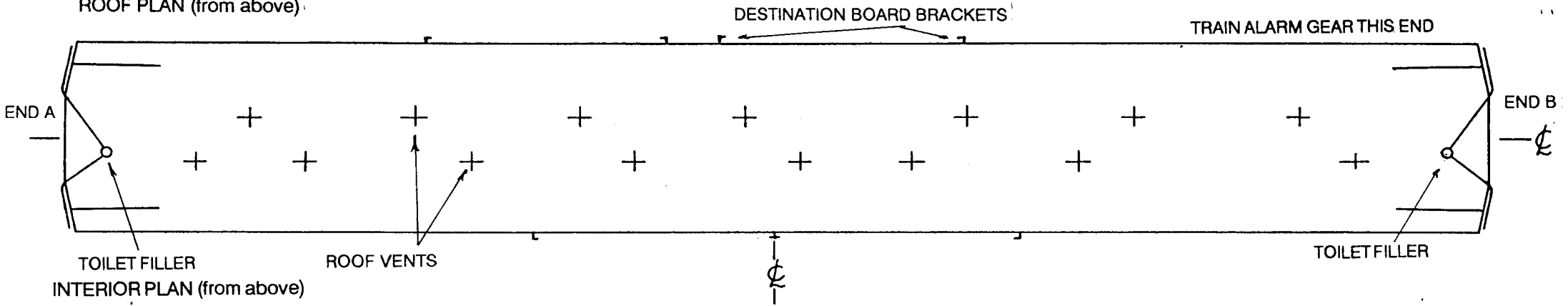
ROOF PLAN (from above)
