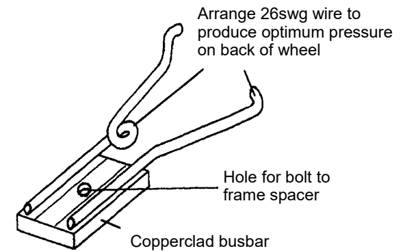
Sketch 3 Suggested pickup arrangement
